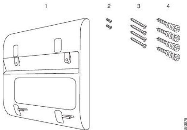
Figure 19: Cisco IP Phone 6800 Series Multiplatform Phones Wall Mount Kit
