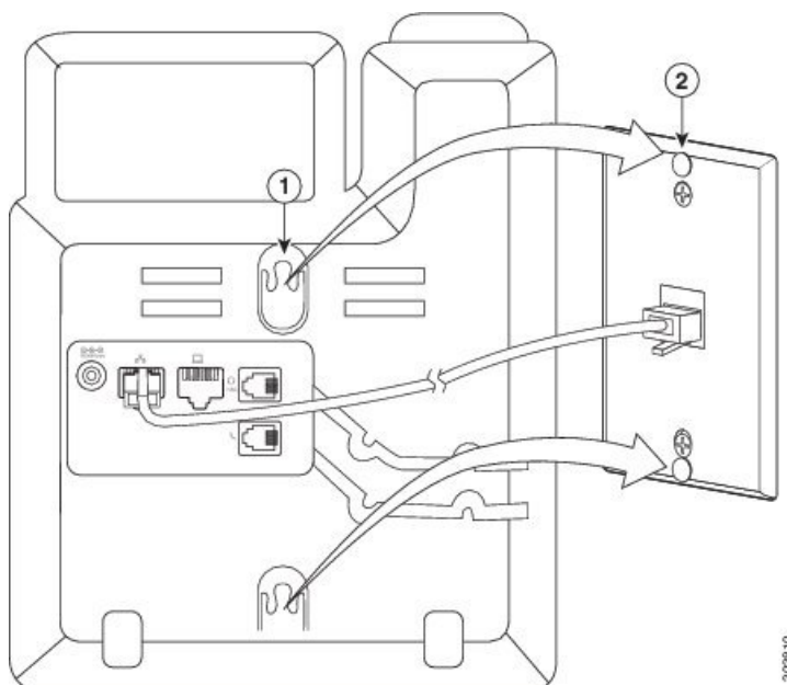
Figure 23: Mounting Holes
