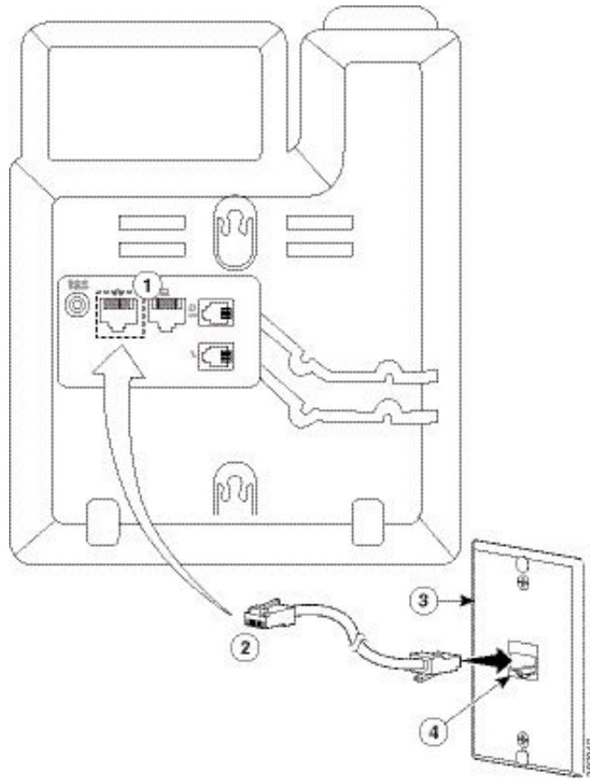
Figure 22: RJ45 Connector in the Wall-Mount Jack
